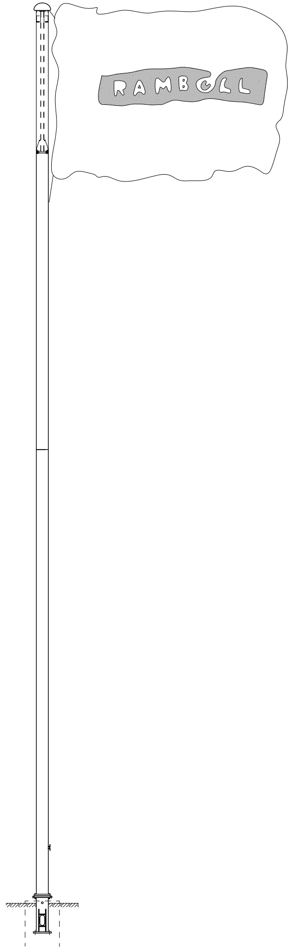
24m Flagpole ø323,9mm, 3,8m Radome Drawing FP-X-005
