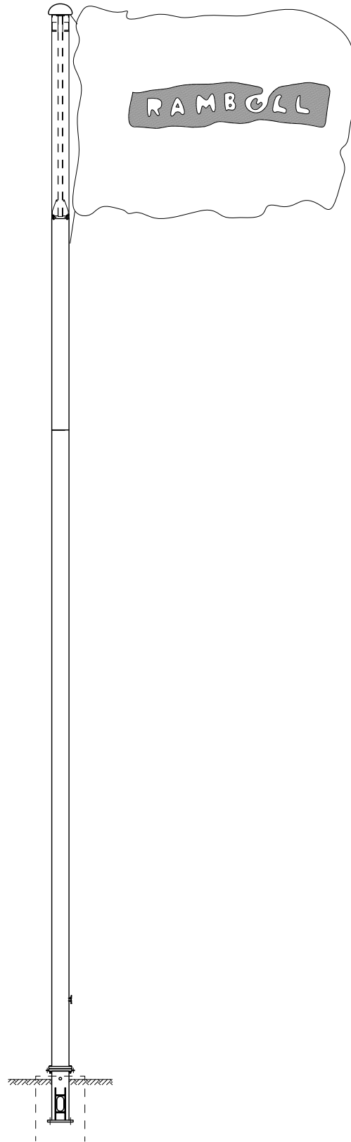
20m Flagpole ø323,9mm, 3,8m Radome Drawing FP-X-004
